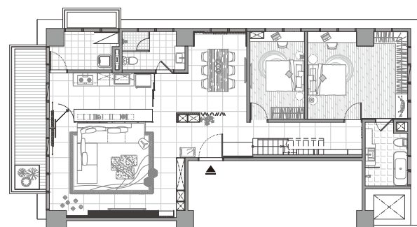
▲ 1st Floor
